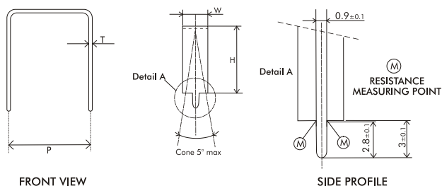
SIDE PROFILE
