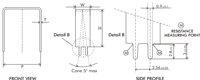
SIDE PROFILE
